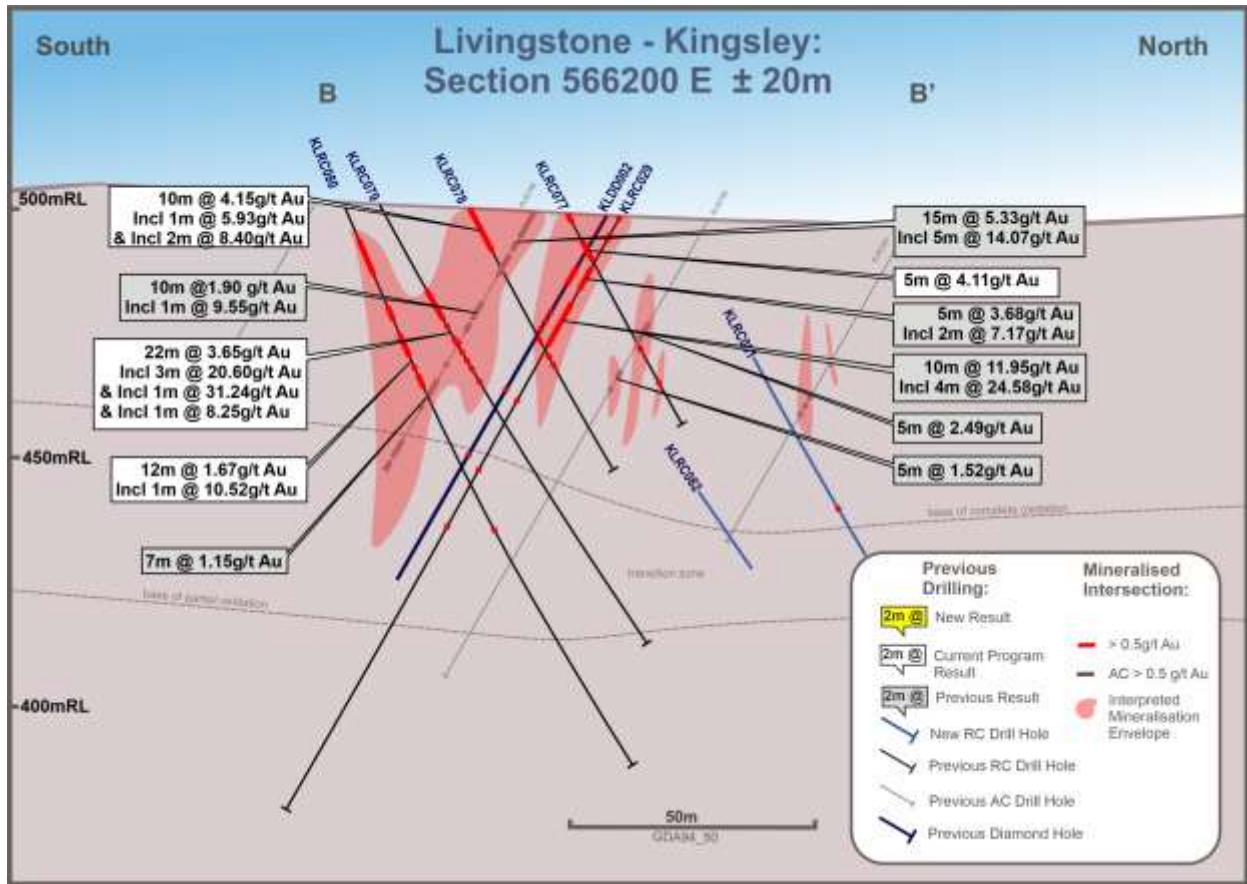
Figure 3: Section B displaying significant mineralised intercepts
