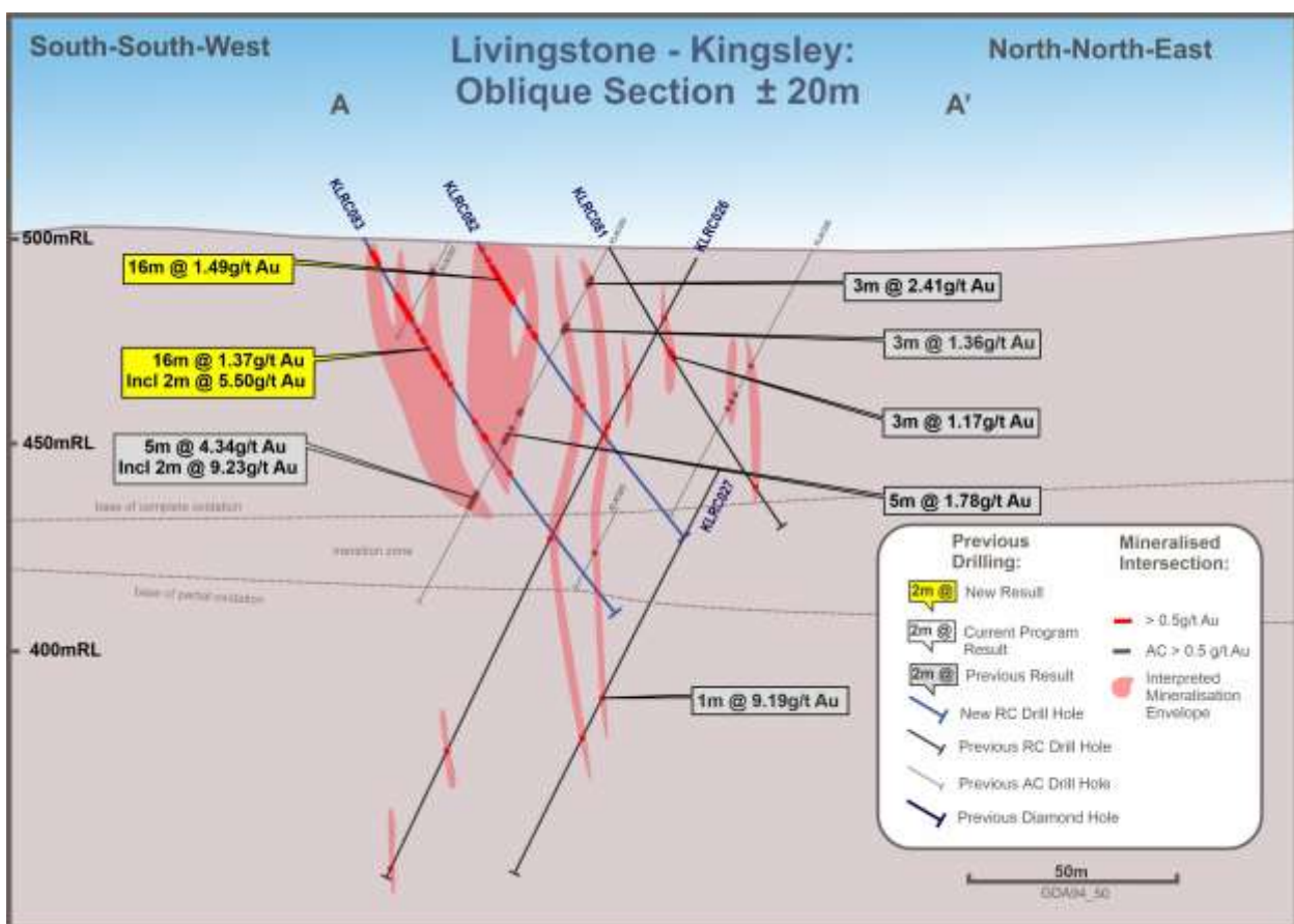
Figure 2: Section A displaying significant mineralised intercepts
