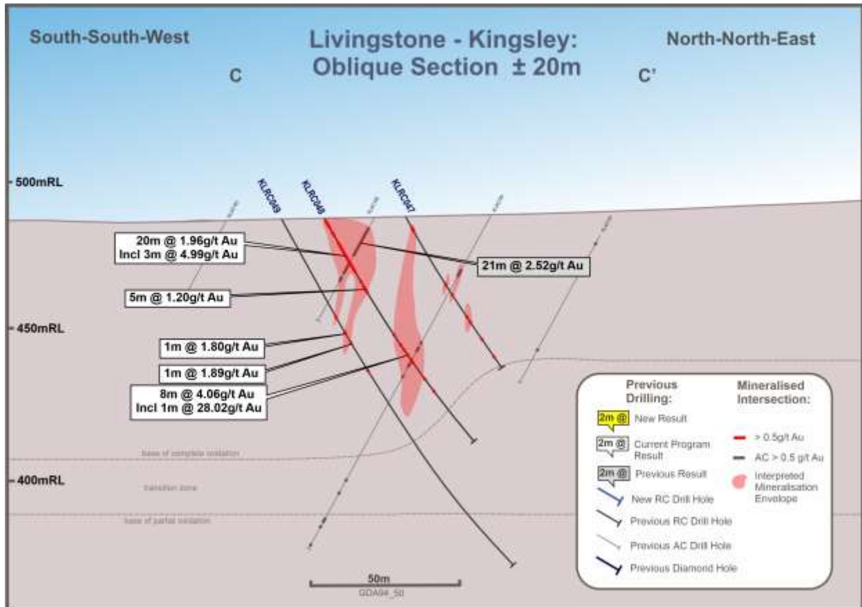
Figure 4: Section C displaying significant mineralised intercepts
